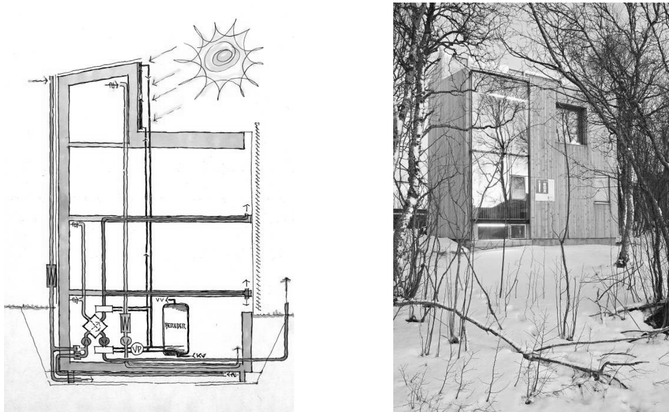
Figure 1: Left: Schematic drawing of the technical system of the I-Box concept (illustration by O. K. Steinsvik). Right: Picture of the completed dwelling at Tromsøya (photo by R. Steinsvik)
