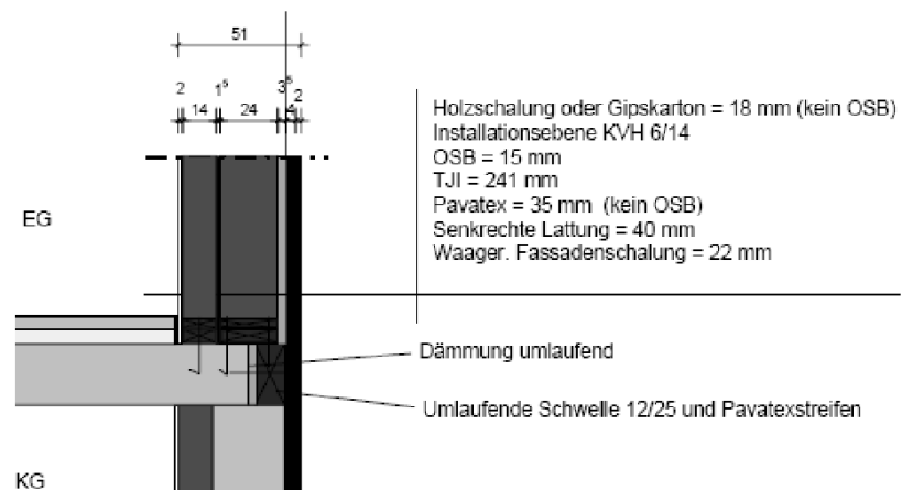
Figure 3: Detail of exterior wall meeting ground floor slab (Illustration by Dipl. Ing. Stephan Blohm)
